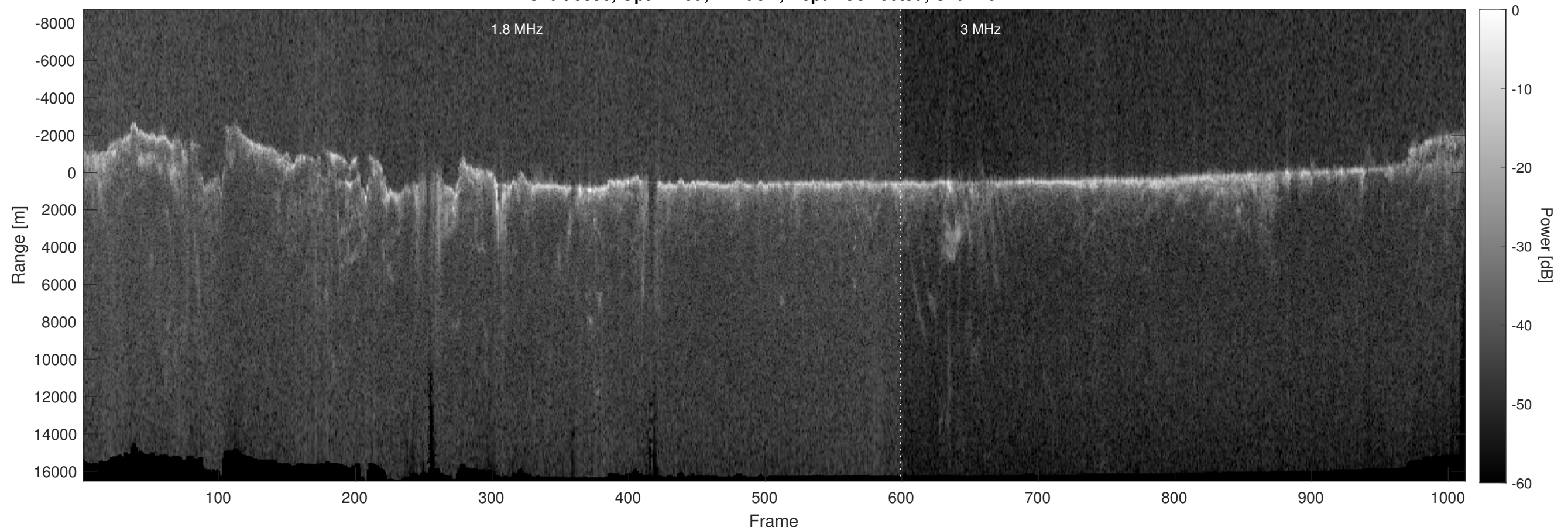
Orbit 3896, Optimized, Window, Depth-Corrected, Channel 2
