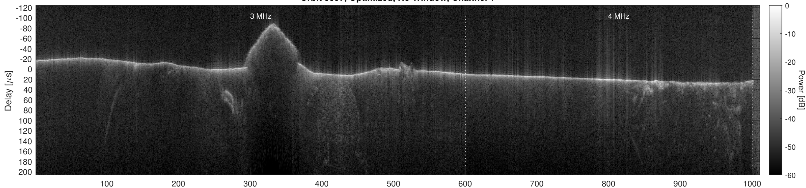
Orbit 3897, Optimized, No Window, Channel 2
