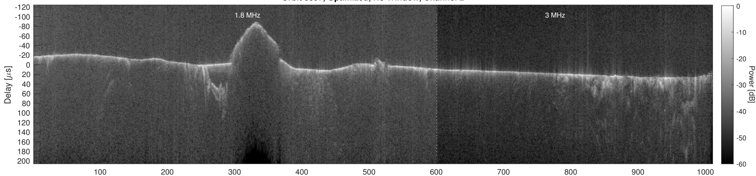
Orbit 3897, Cluttergram
