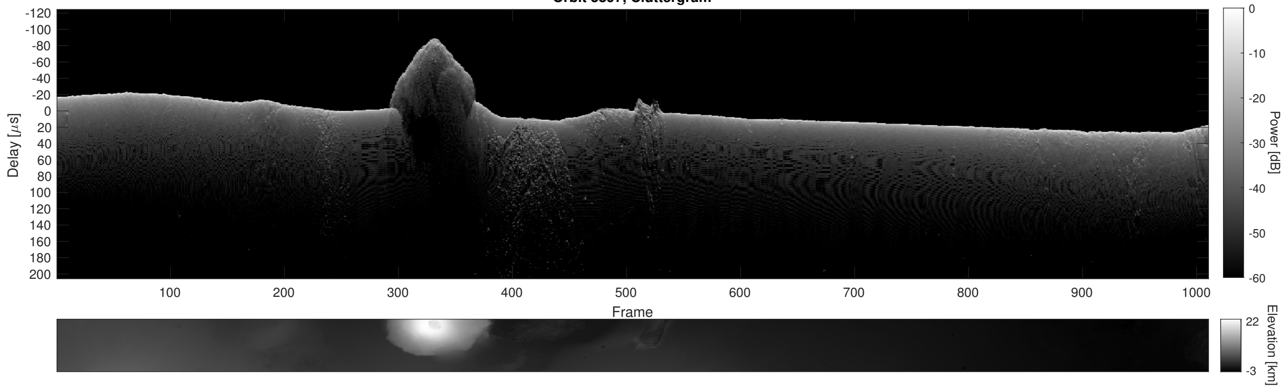
Orbit 3897, Cluttergram
