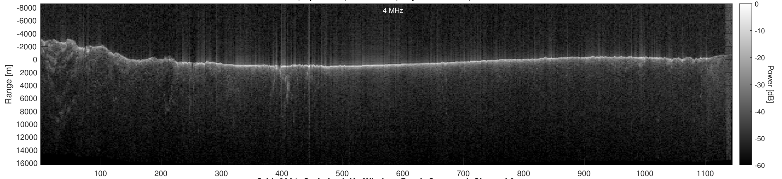
Orbit 3901, Optimized, No Window, Depth-Corrected, Channel 2
