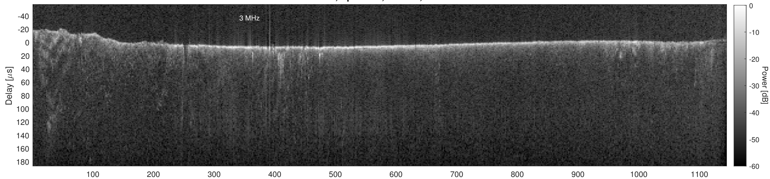
Orbit 3901, Cluttergram
