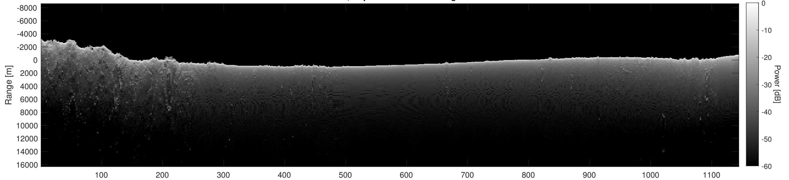
Orbit 3901, Depth-Corrected Cluttergram
