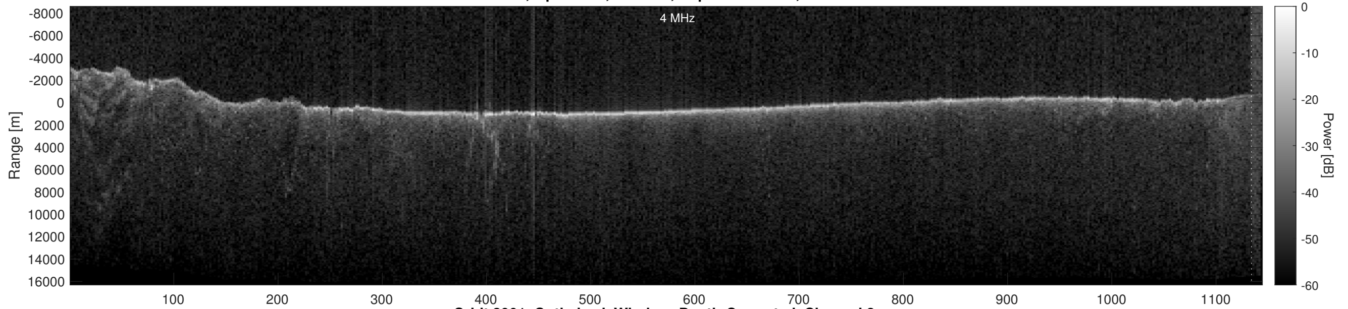
Orbit 3901, Optimized, Window, Depth-Corrected, Channel 2
