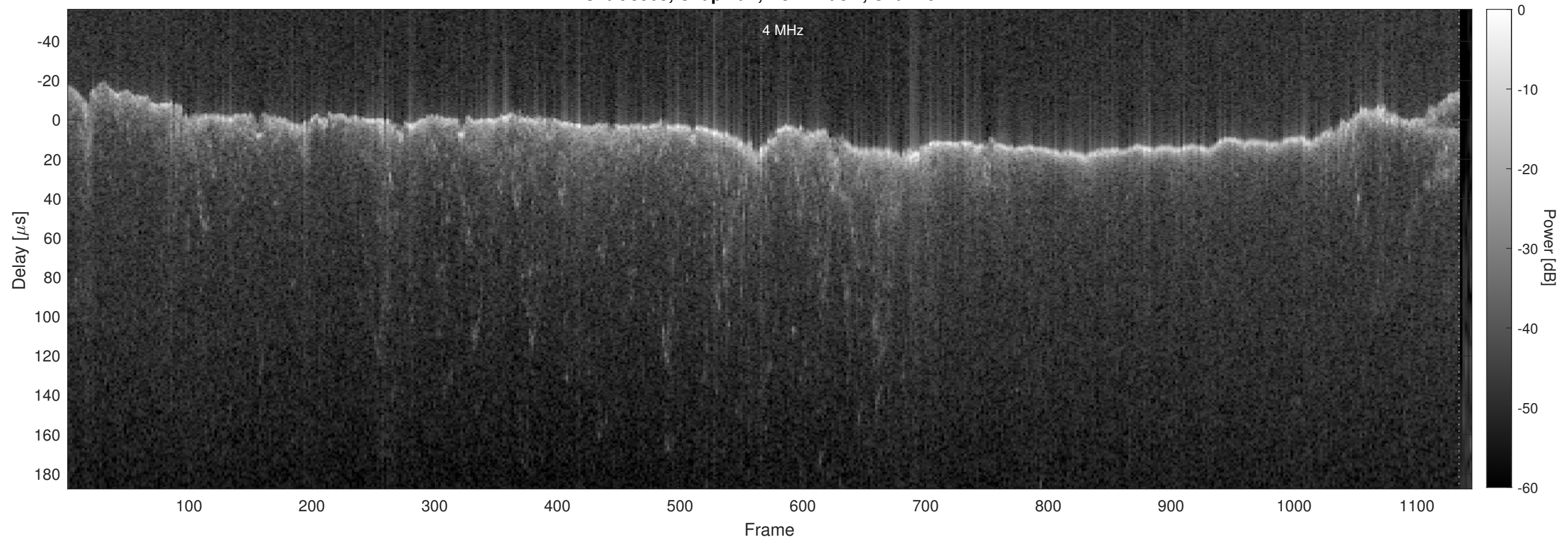
Orbit 3903, Chapman, No Window, Channel 2
