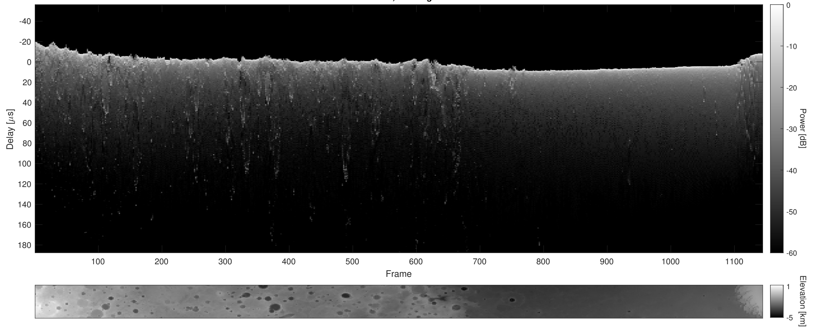
Orbit 3903, Cluttergram
