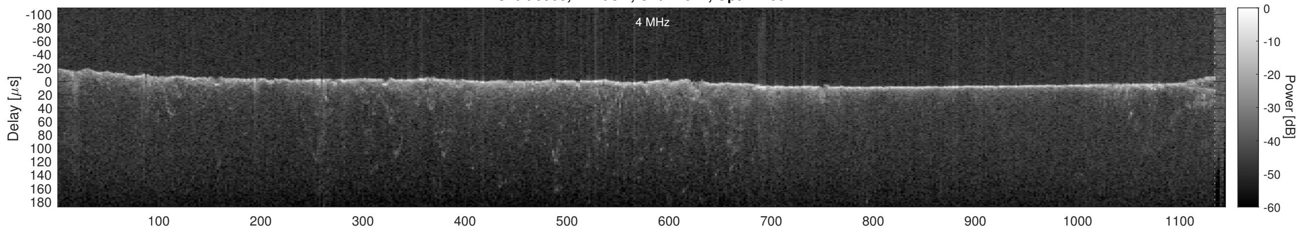
Orbit 3903, Cluttergram
