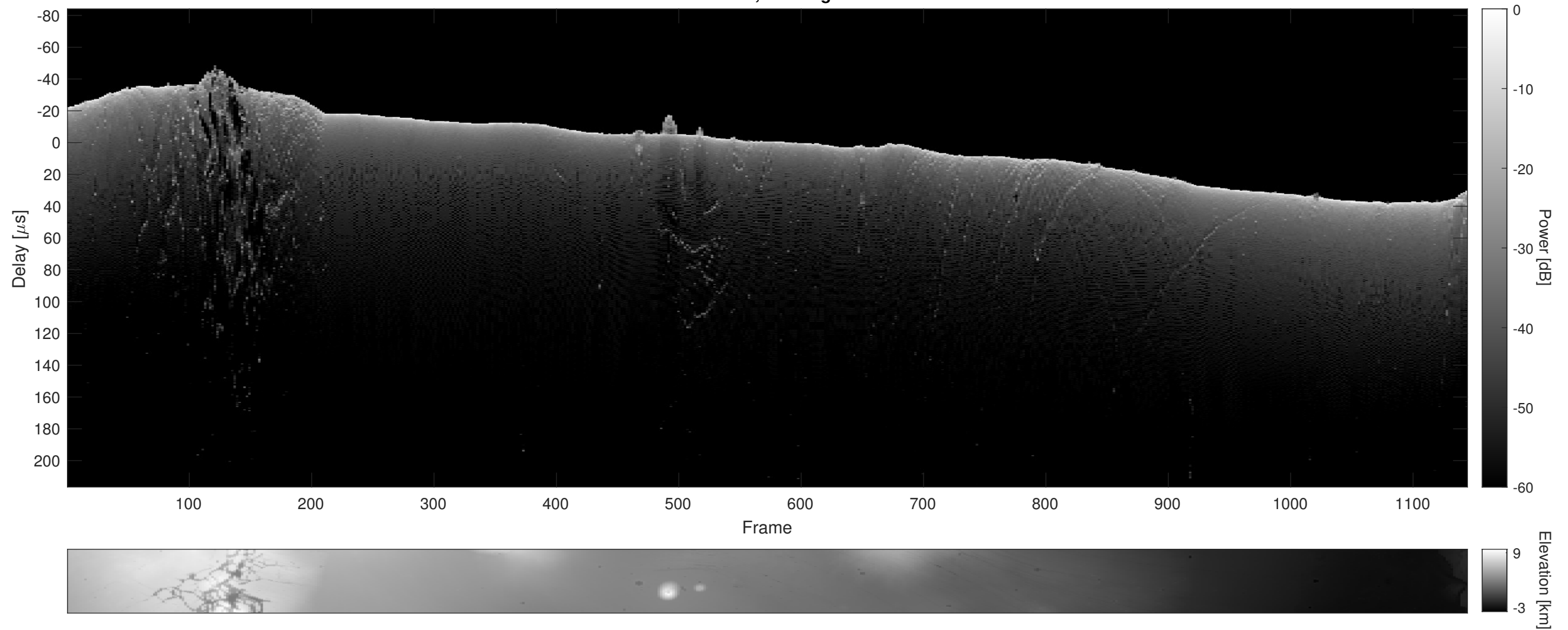
Orbit 3904, Cluttergram
