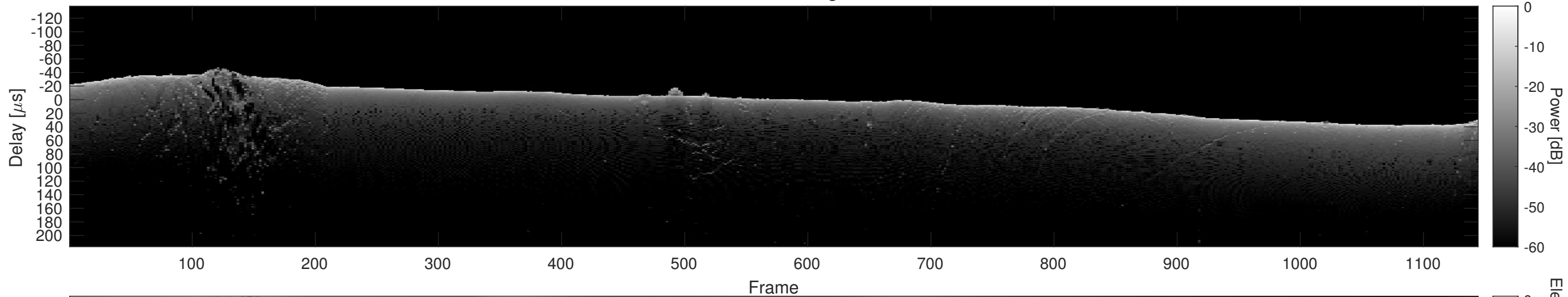
Orbit 3904, Cluttergram
