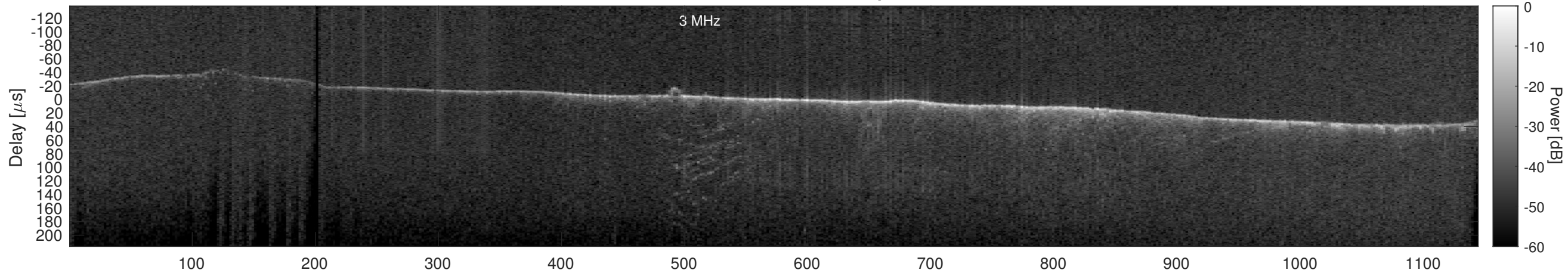
Orbit 3904, Cluttergram
