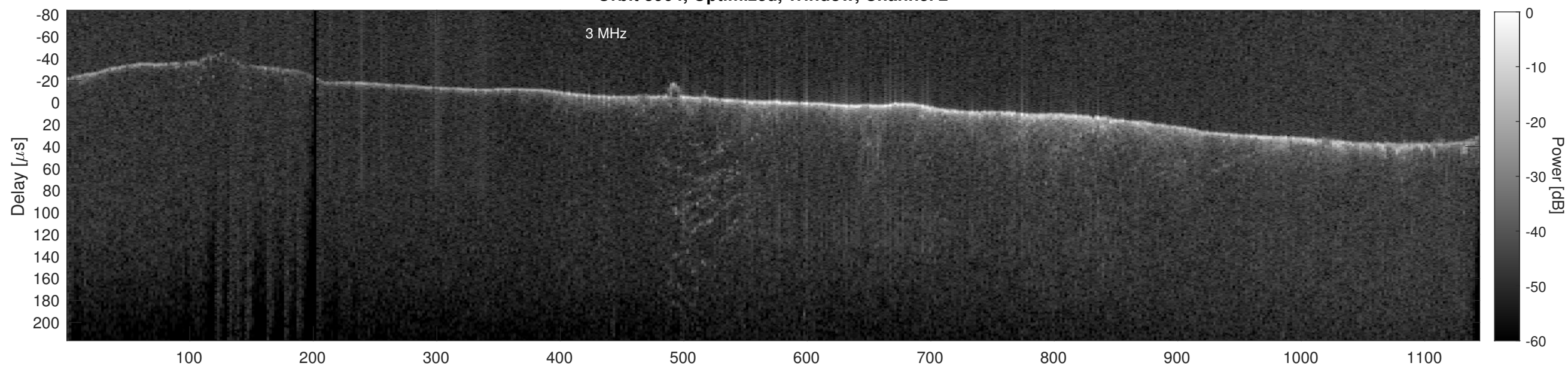
Orbit 3904, Cluttergram
