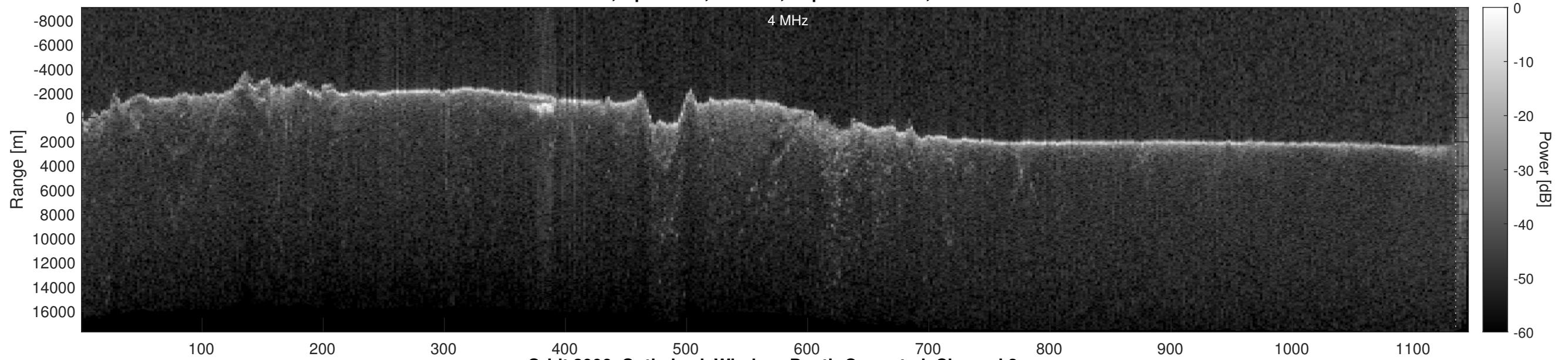
Orbit 3906, Optimized, Window, Depth-Corrected, Channel 2
