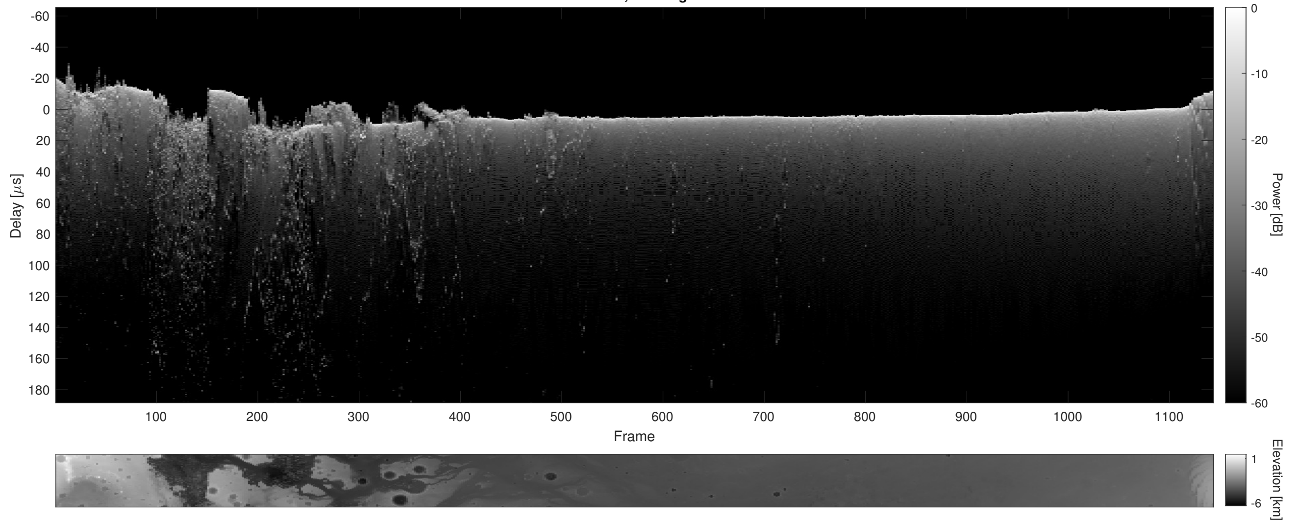
Orbit 3907, Cluttergram
