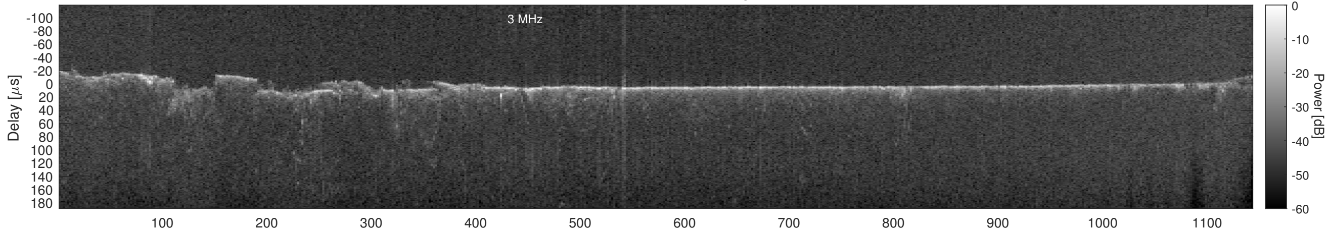
Orbit 3907, Cluttergram
