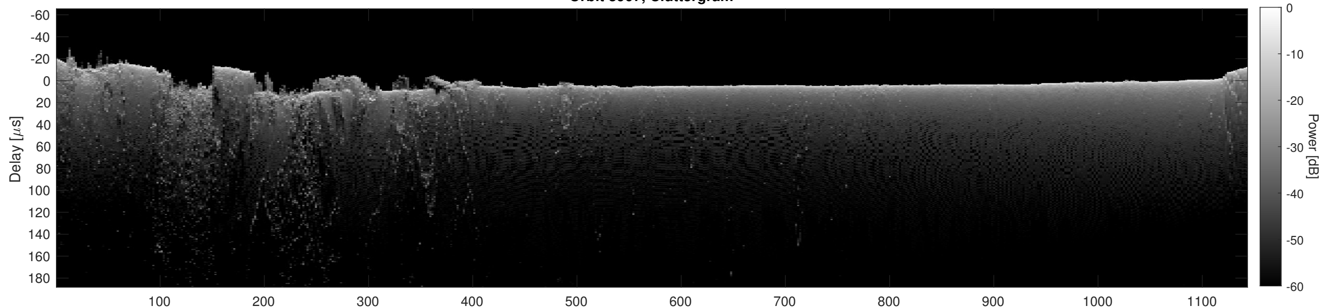
Orbit 3907, Cluttergram
