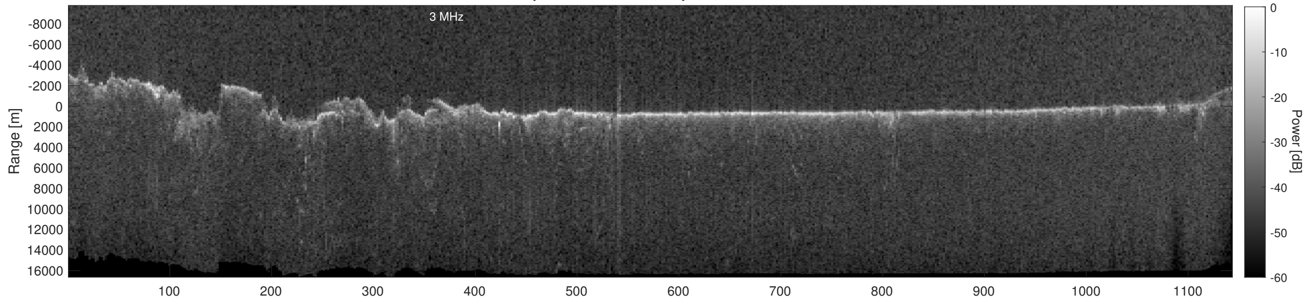
Orbit 3907, Depth-Corrected Cluttergram
