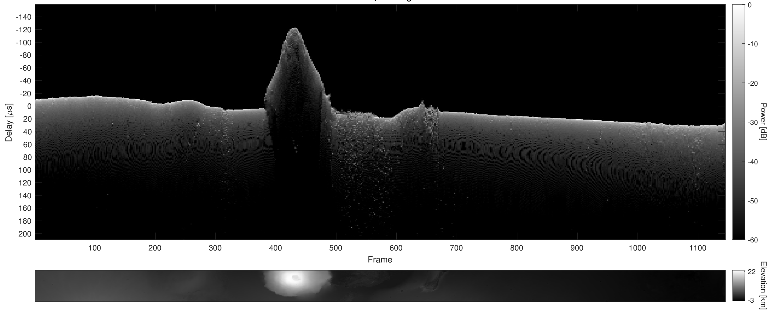
Orbit 3908, Cluttergram
