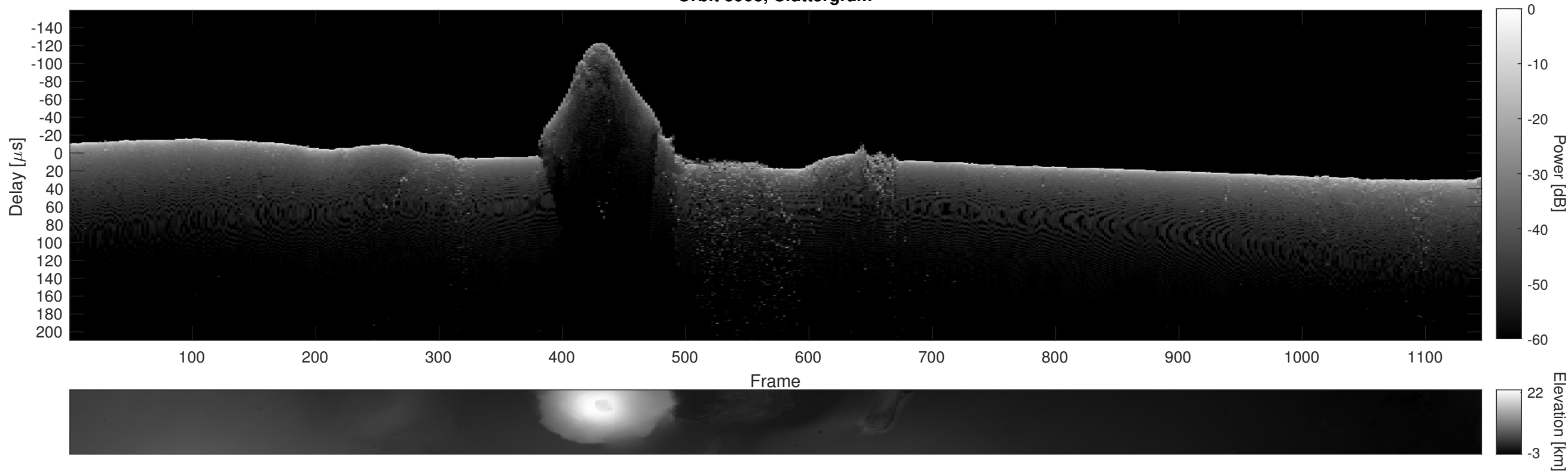
Orbit 3908, Cluttergram
