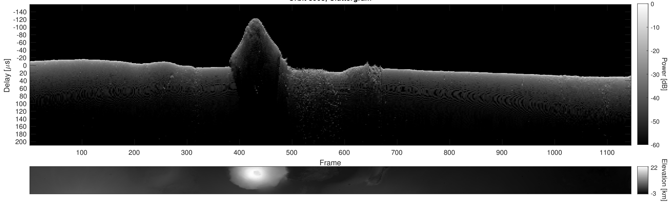
Orbit 3908, Cluttergram
