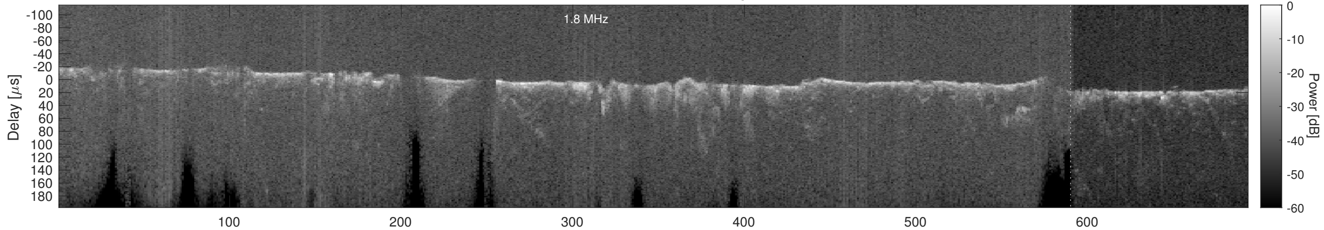
Orbit 3910, Cluttergram
