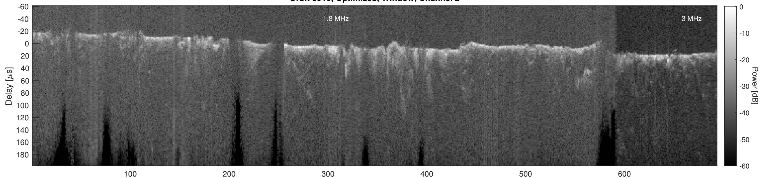
Orbit 3910, Cluttergram
