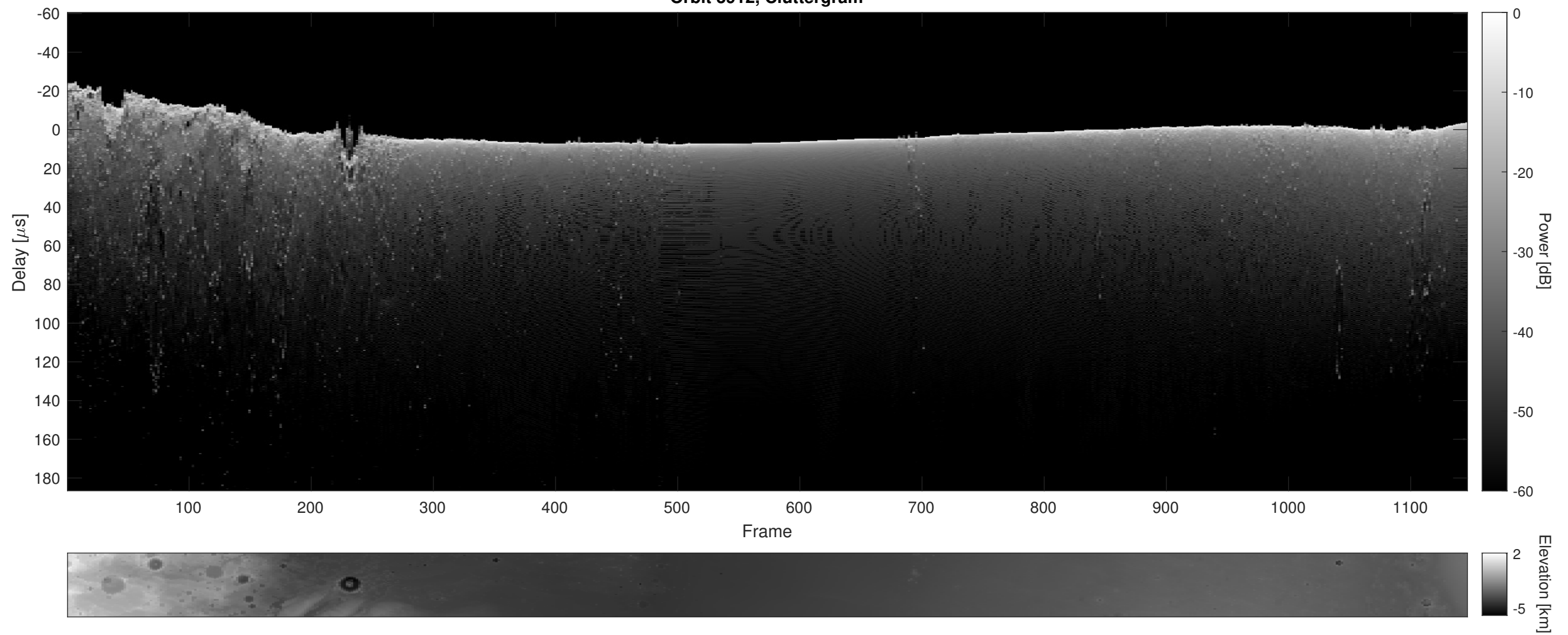
Orbit 3912, Cluttergram
