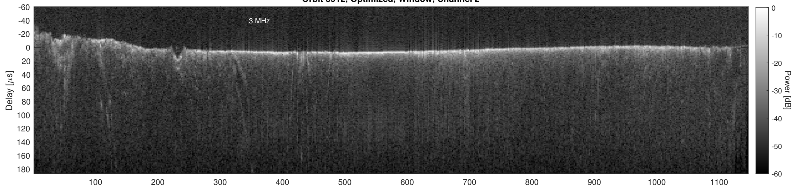
Orbit 3912, Cluttergram
