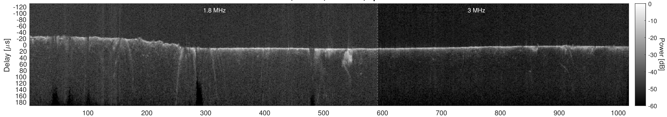
Orbit 3913, Cluttergram
