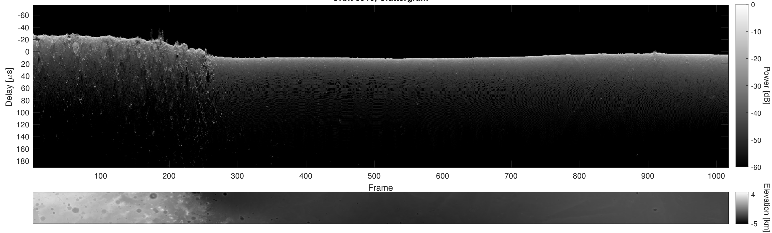
Orbit 3913, Cluttergram
