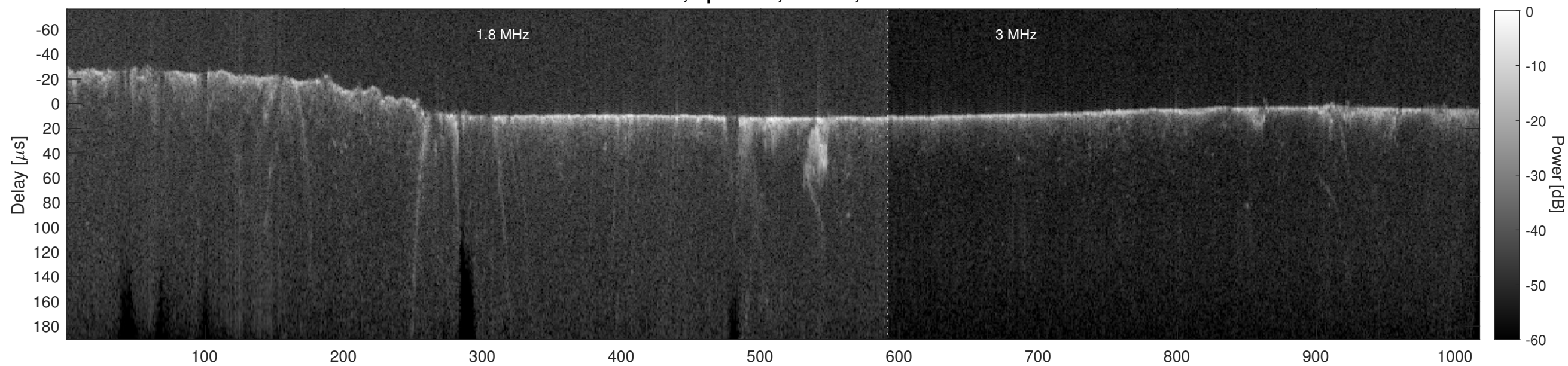
Orbit 3913, Cluttergram
