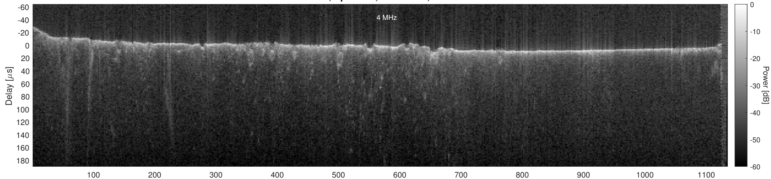
Orbit 3914, Optimized, No Window, Channel 2
