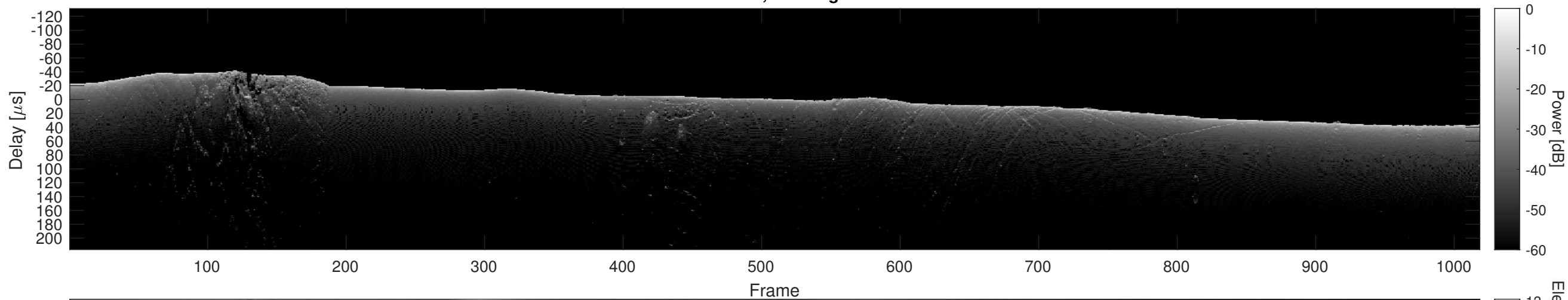
Orbit 3915, Cluttergram
