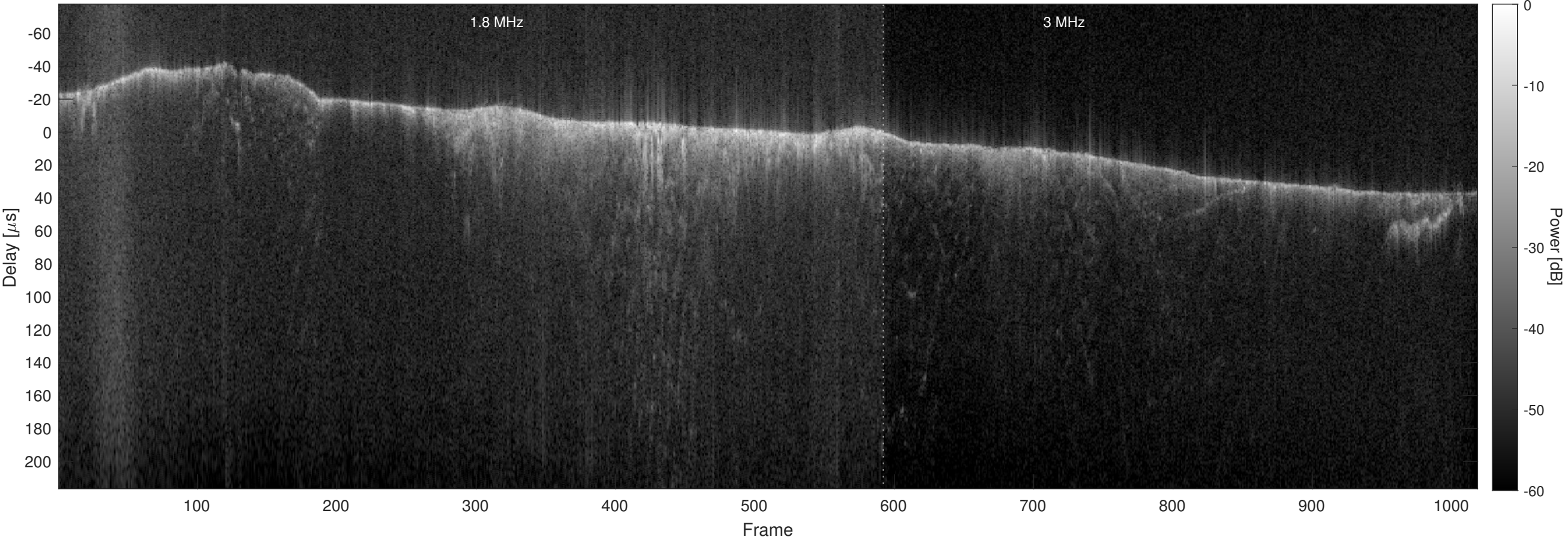
Orbit 3915, Optimized, No Window, Channel 2
