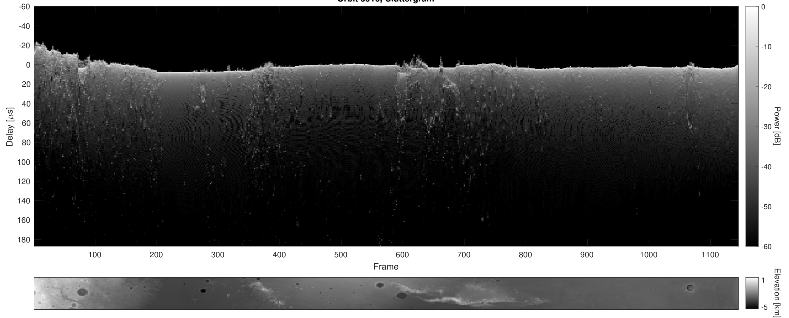
Orbit 3916, Cluttergram
