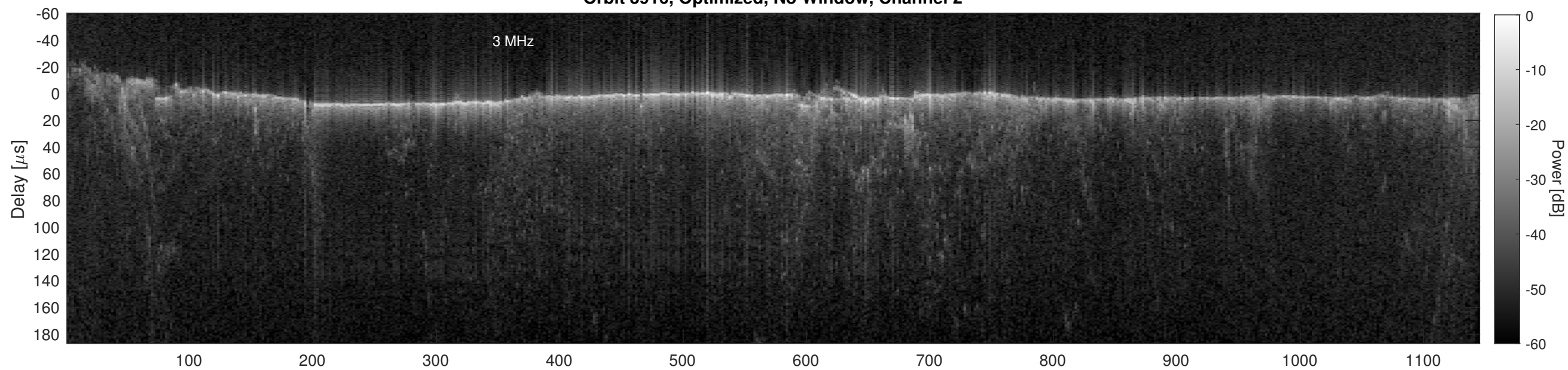
Orbit 3916, Cluttergram
