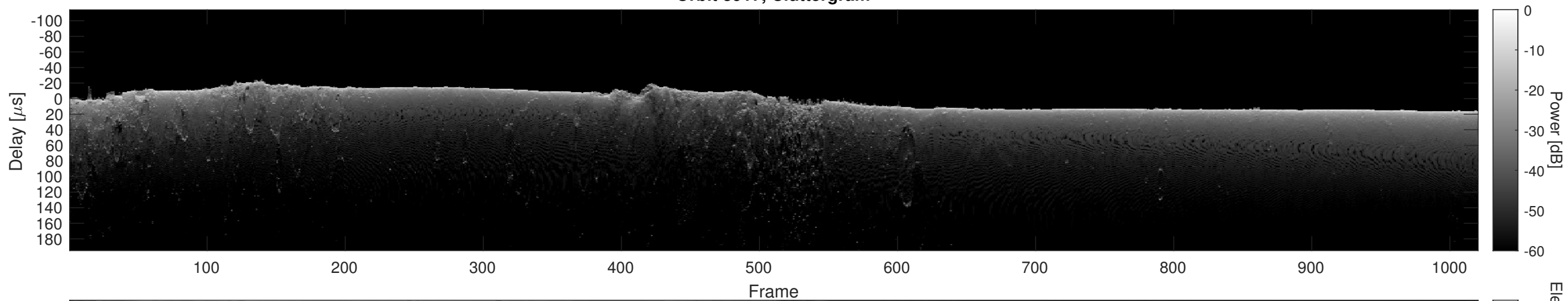
Orbit 3917, Cluttergram
