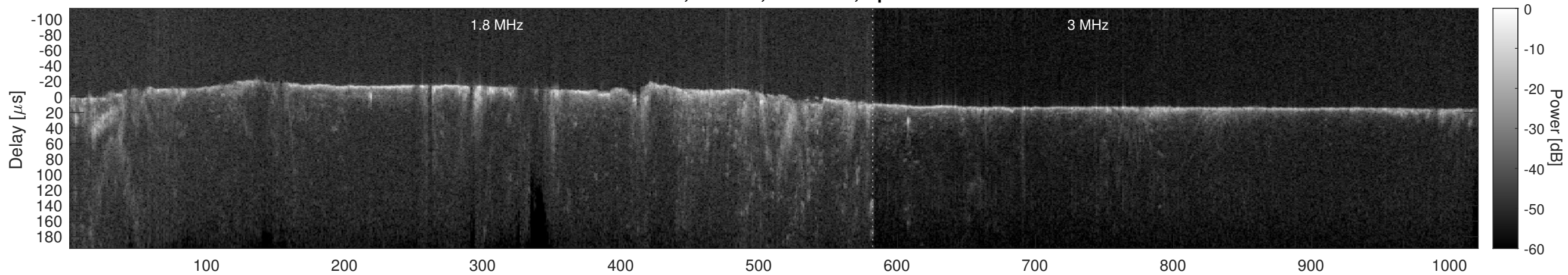
Orbit 3917, Cluttergram
