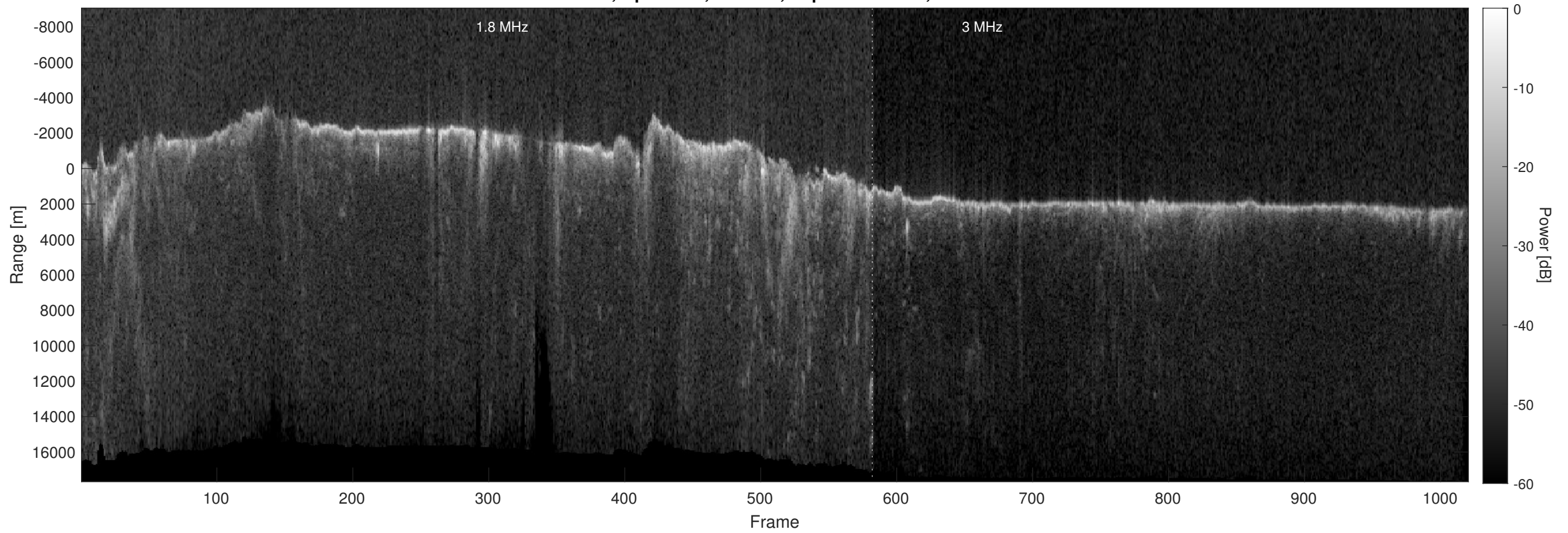
Orbit 3917, Optimized, Window, Depth-Corrected, Channel 2
