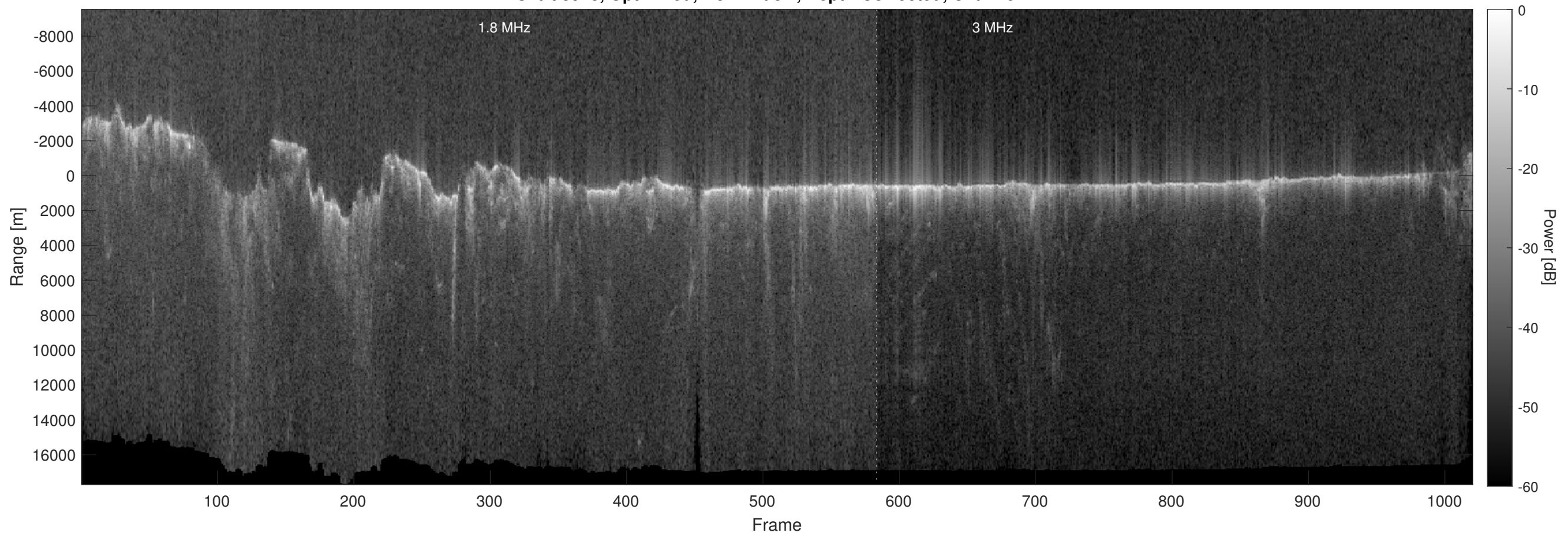
Orbit 3918, Optimized, No Window, Depth-Corrected, Channel 2
