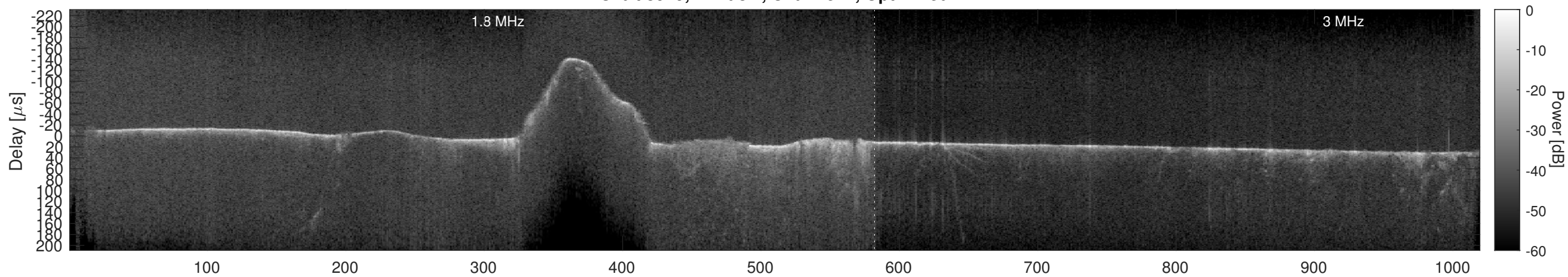
Orbit 3919, Cluttergram
