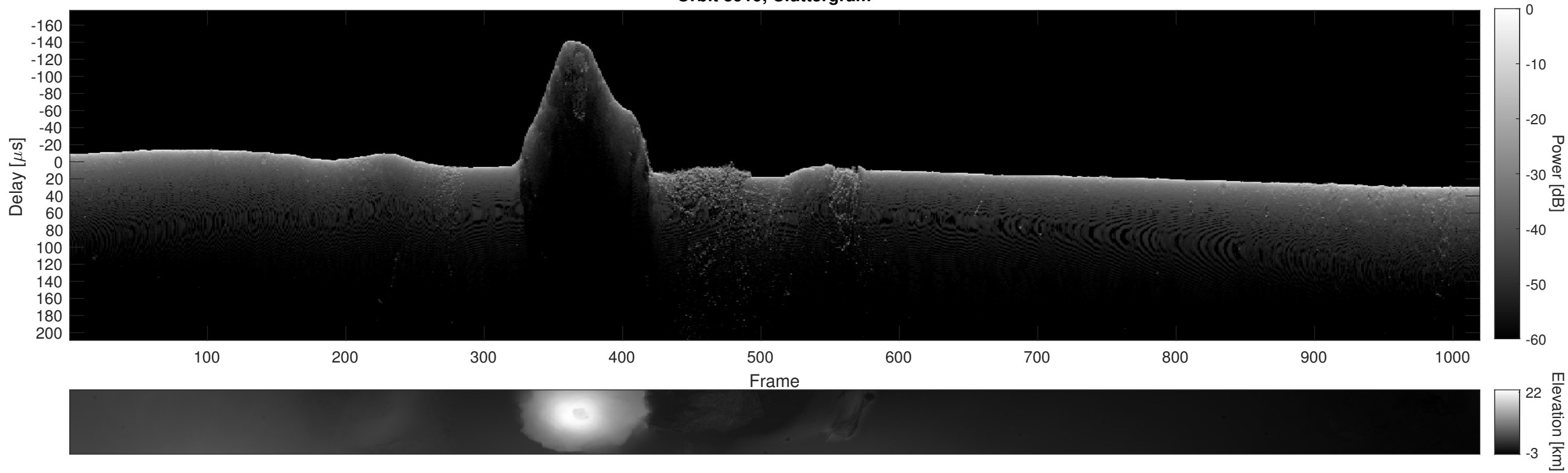
Orbit 3919, Cluttergram
