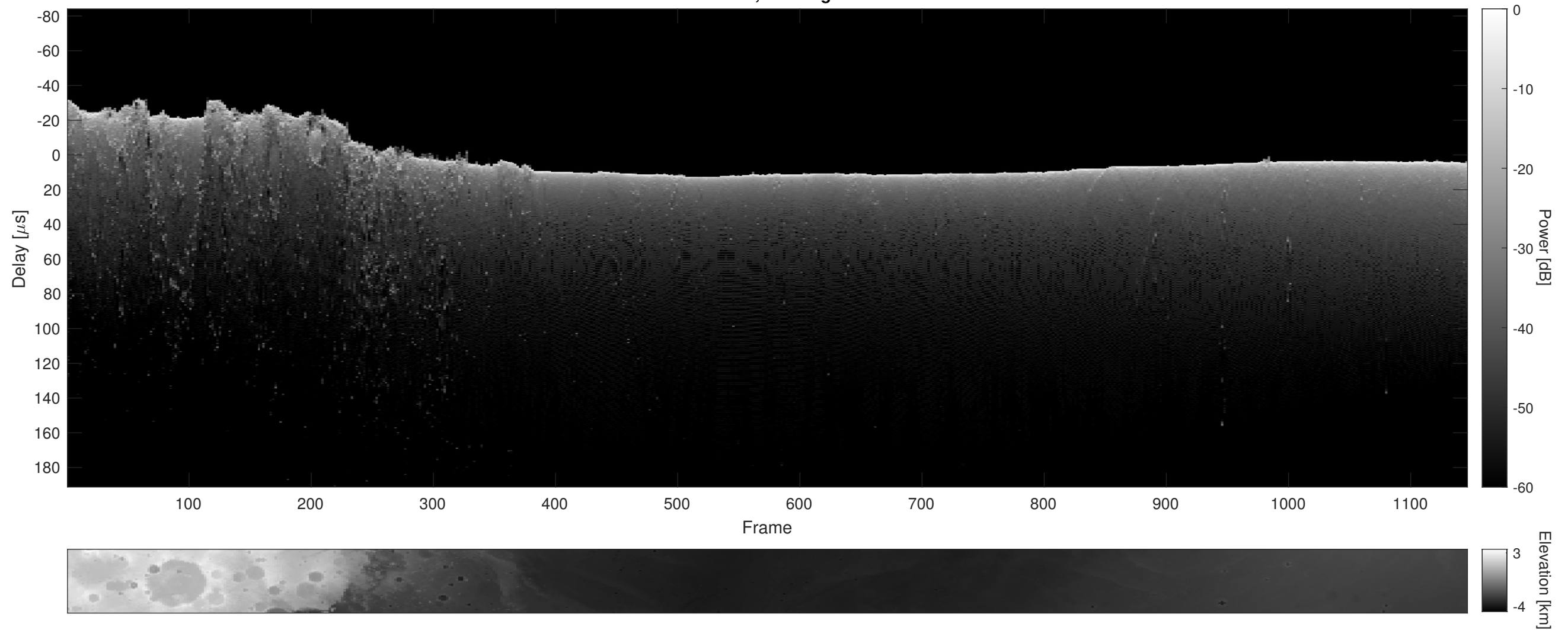
Orbit 3920, Cluttergram
