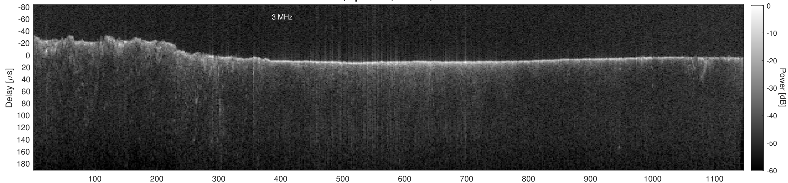
Orbit 3920, Cluttergram
