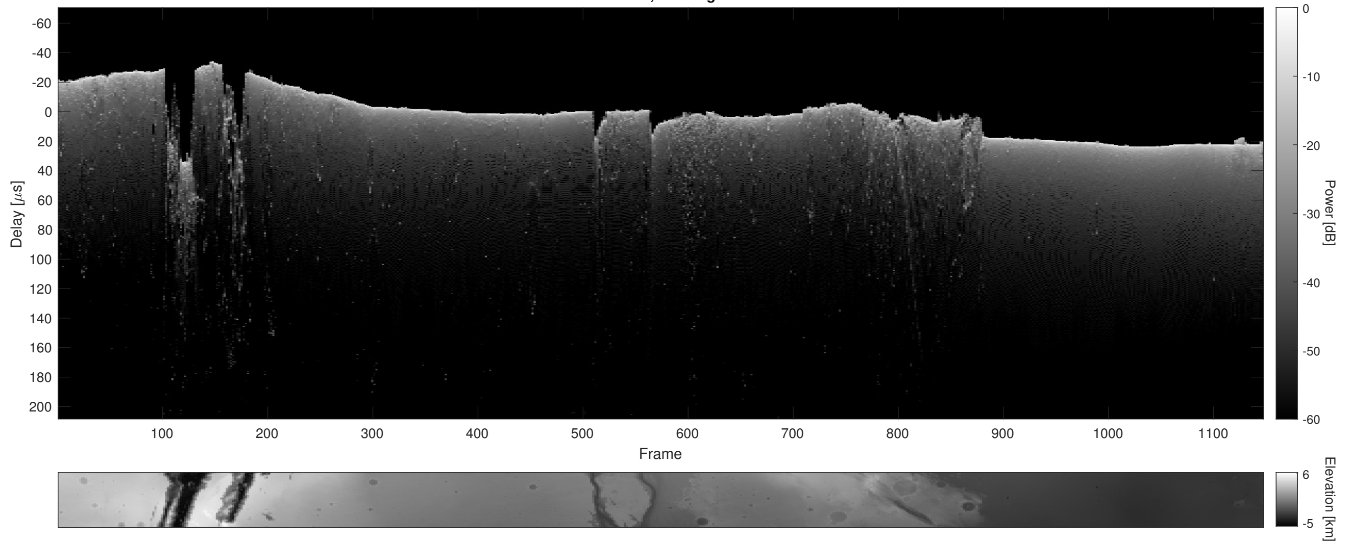
Orbit 3922, Cluttergram
