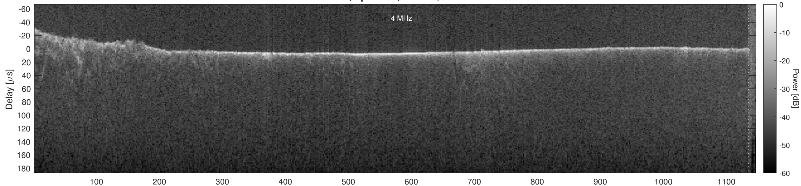
Orbit 3923, Optimized, Window, Channel 2
