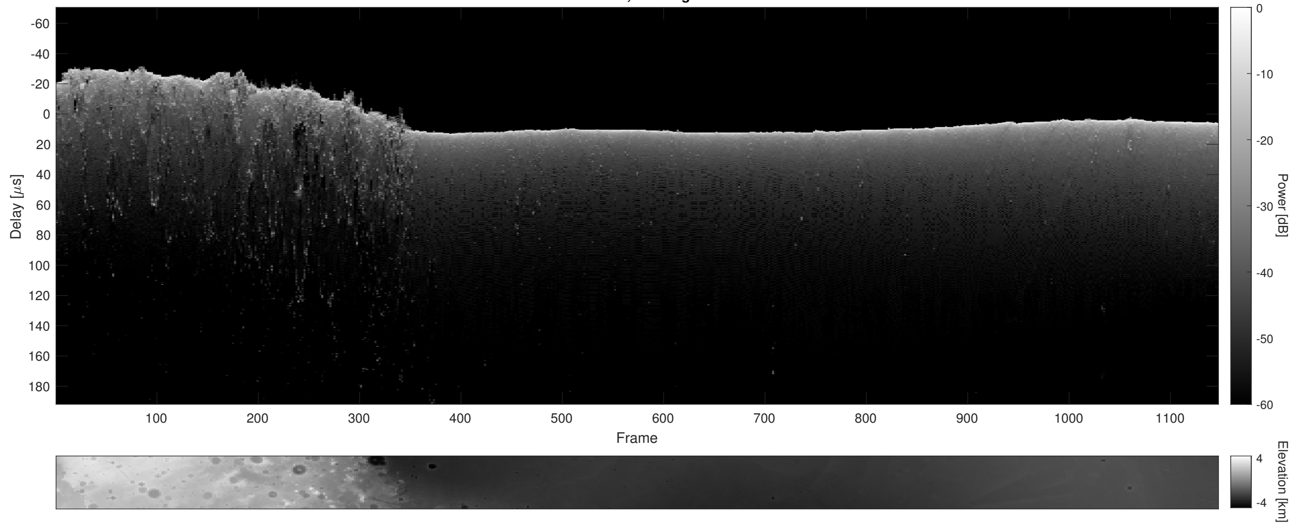
Orbit 3924, Cluttergram
