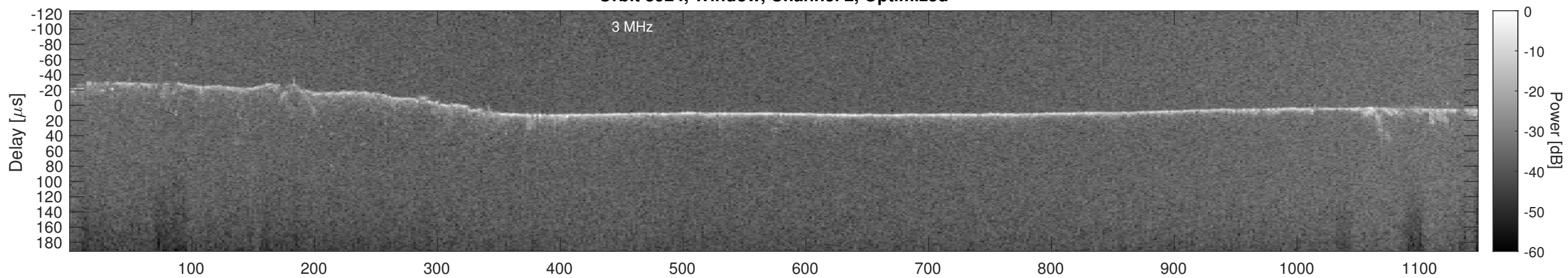
Orbit 3924, Cluttergram
