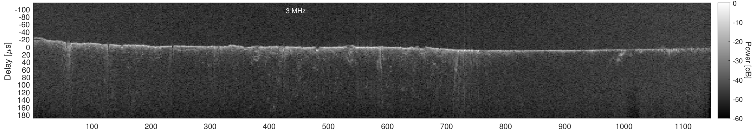
Orbit 3925, Cluttergram
