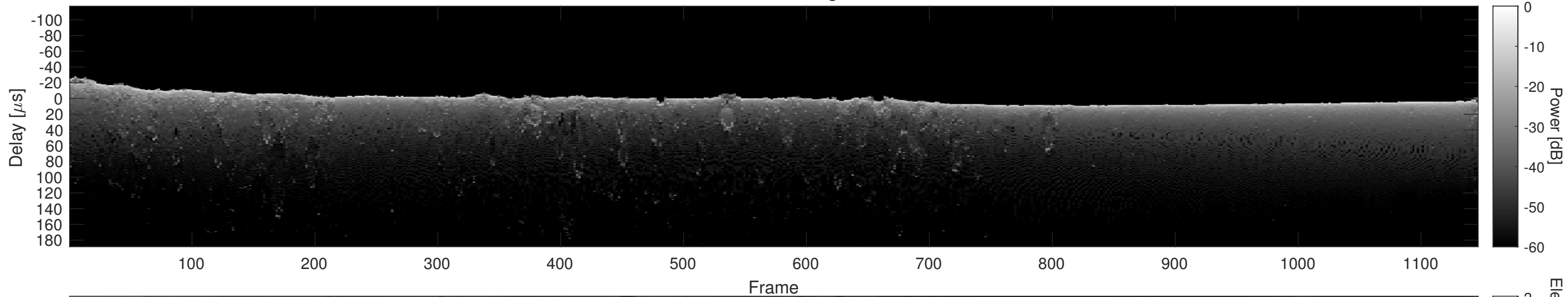
Orbit 3925, Cluttergram
