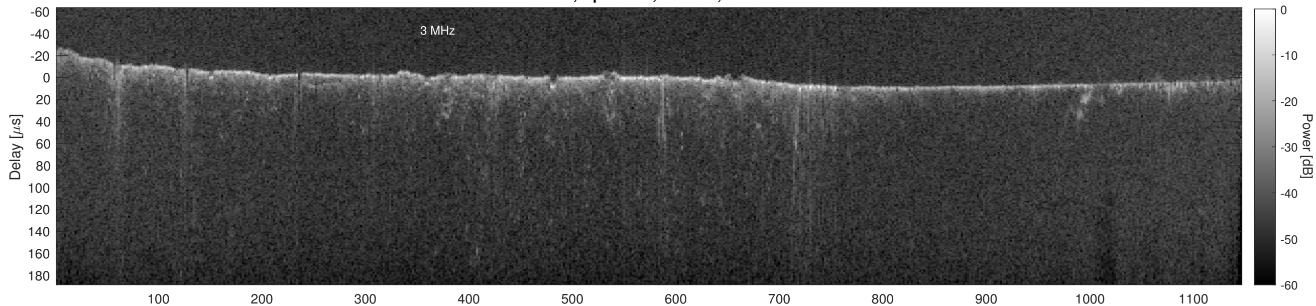
Orbit 3925, Cluttergram
