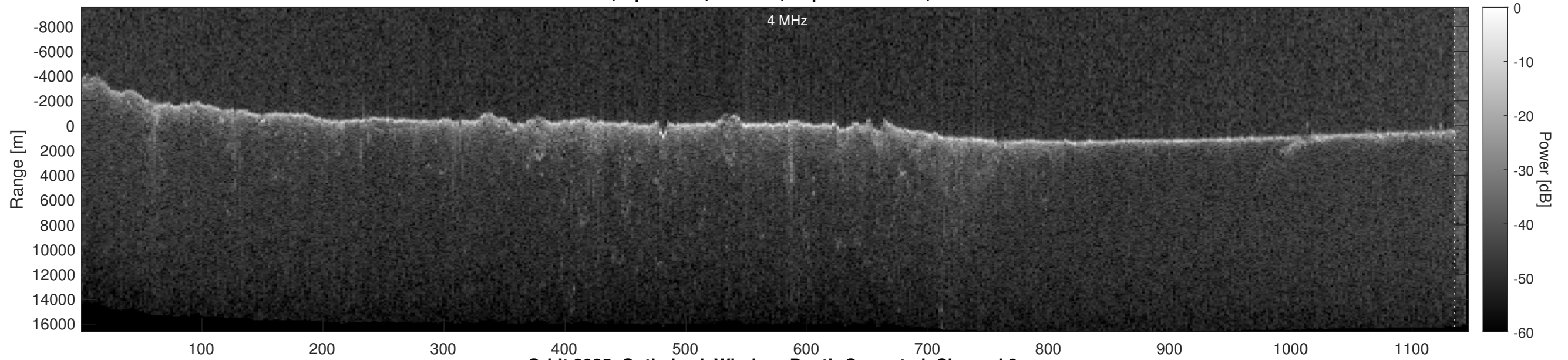
Orbit 3925, Optimized, Window, Depth-Corrected, Channel 2
