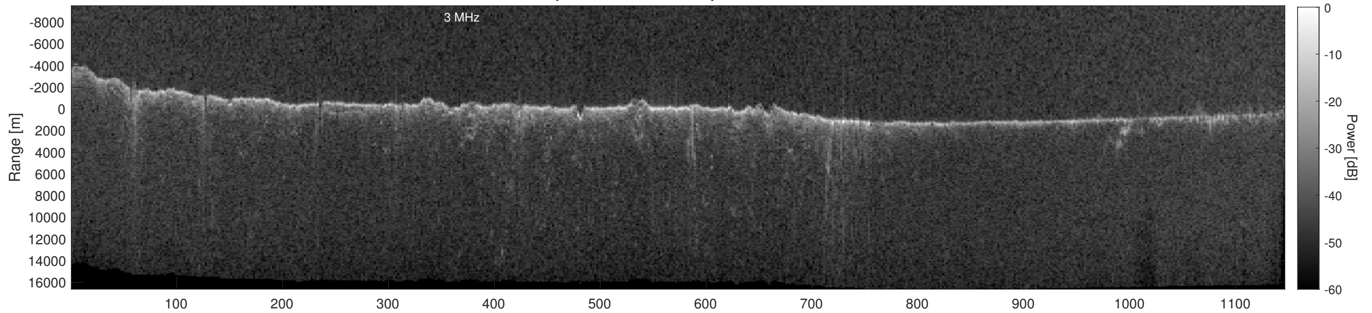
Orbit 3925, Depth-Corrected Cluttergram
