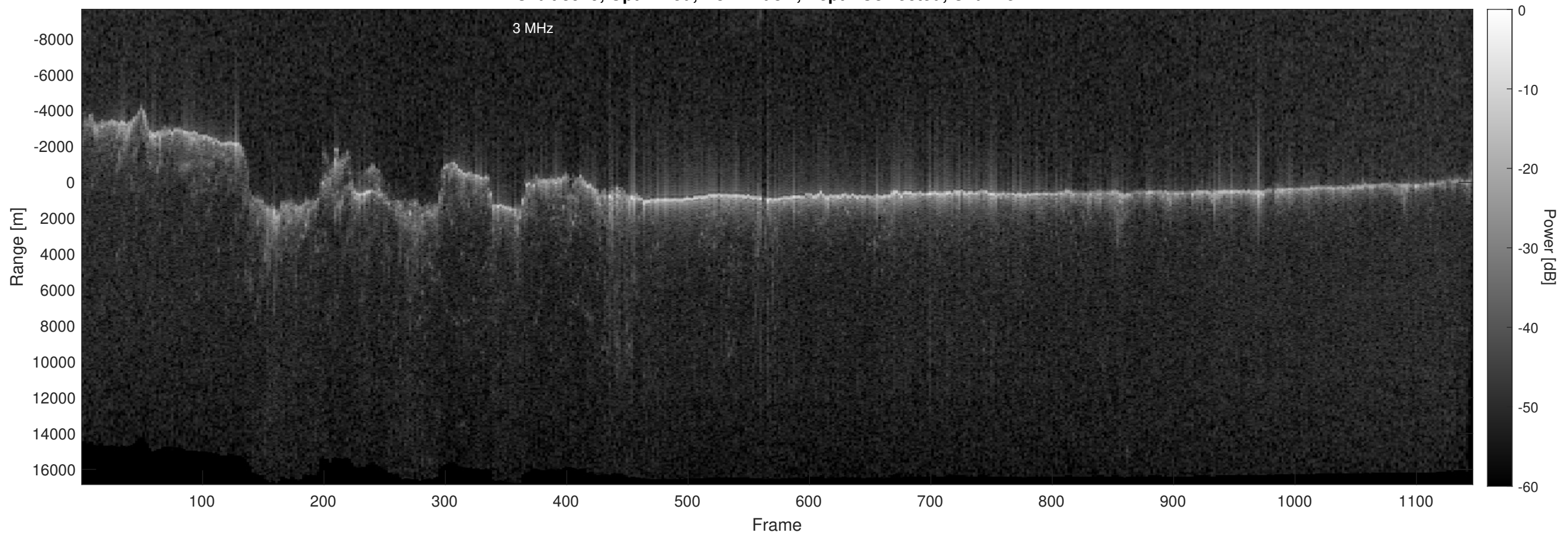
Orbit 3929, Optimized, No Window, Depth-Corrected, Channel 2
