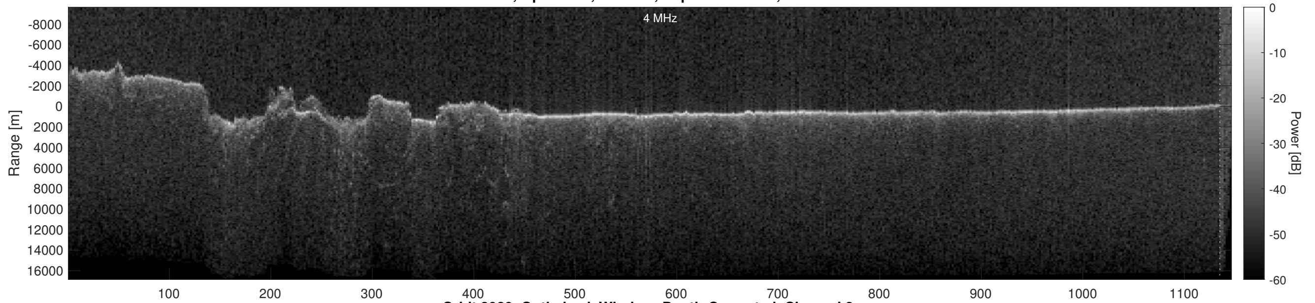
Orbit 3929, Optimized, Window, Depth-Corrected, Channel 2
