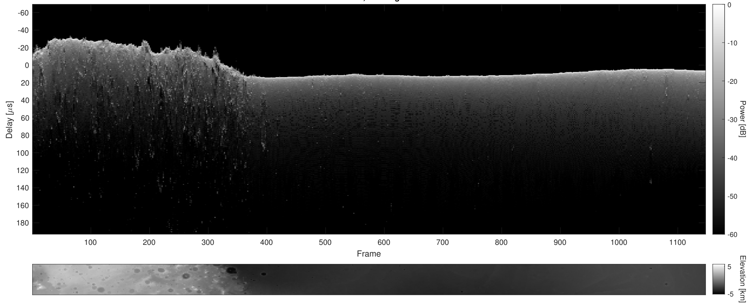
Orbit 3935, Cluttergram
