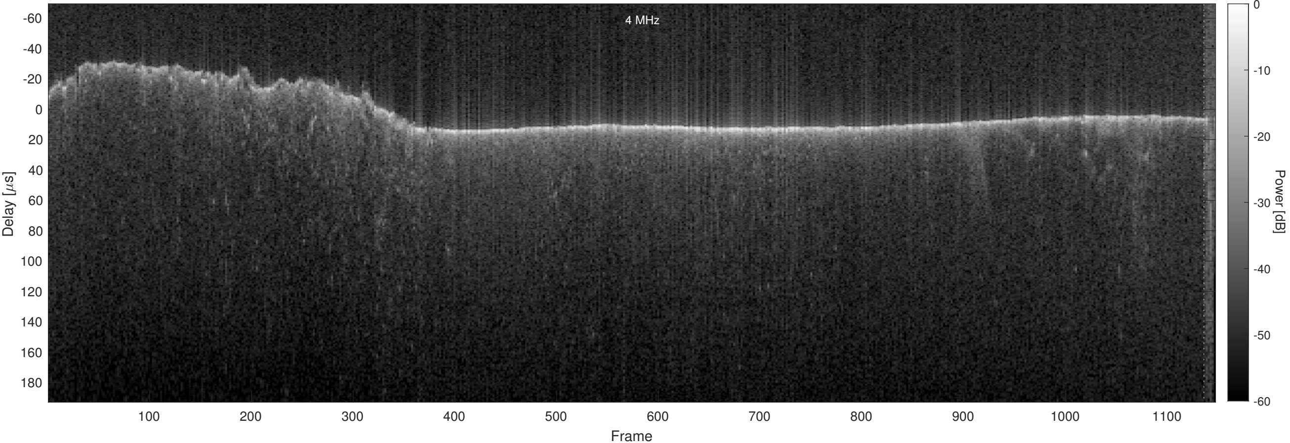
Orbit 3935, Optimized, No Window, Channel 2
