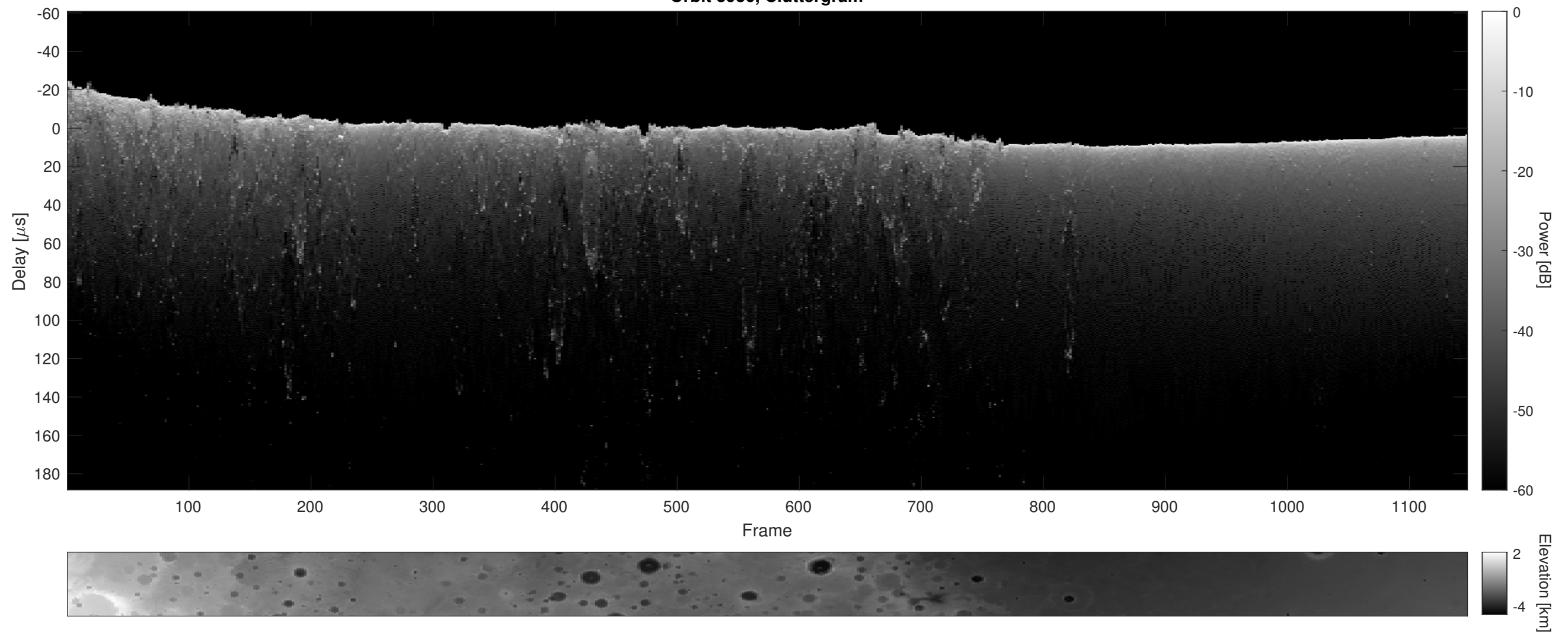
Orbit 3936, Cluttergram
