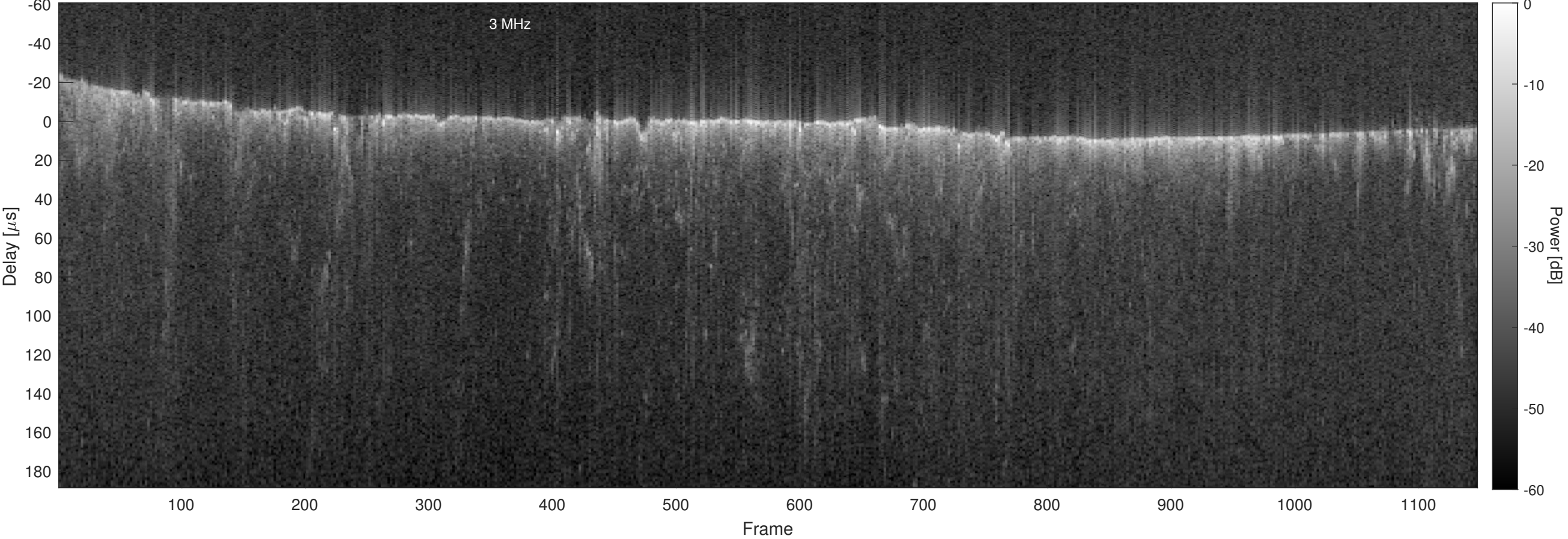
Orbit 3936, Optimized, No Window, Channel 2
